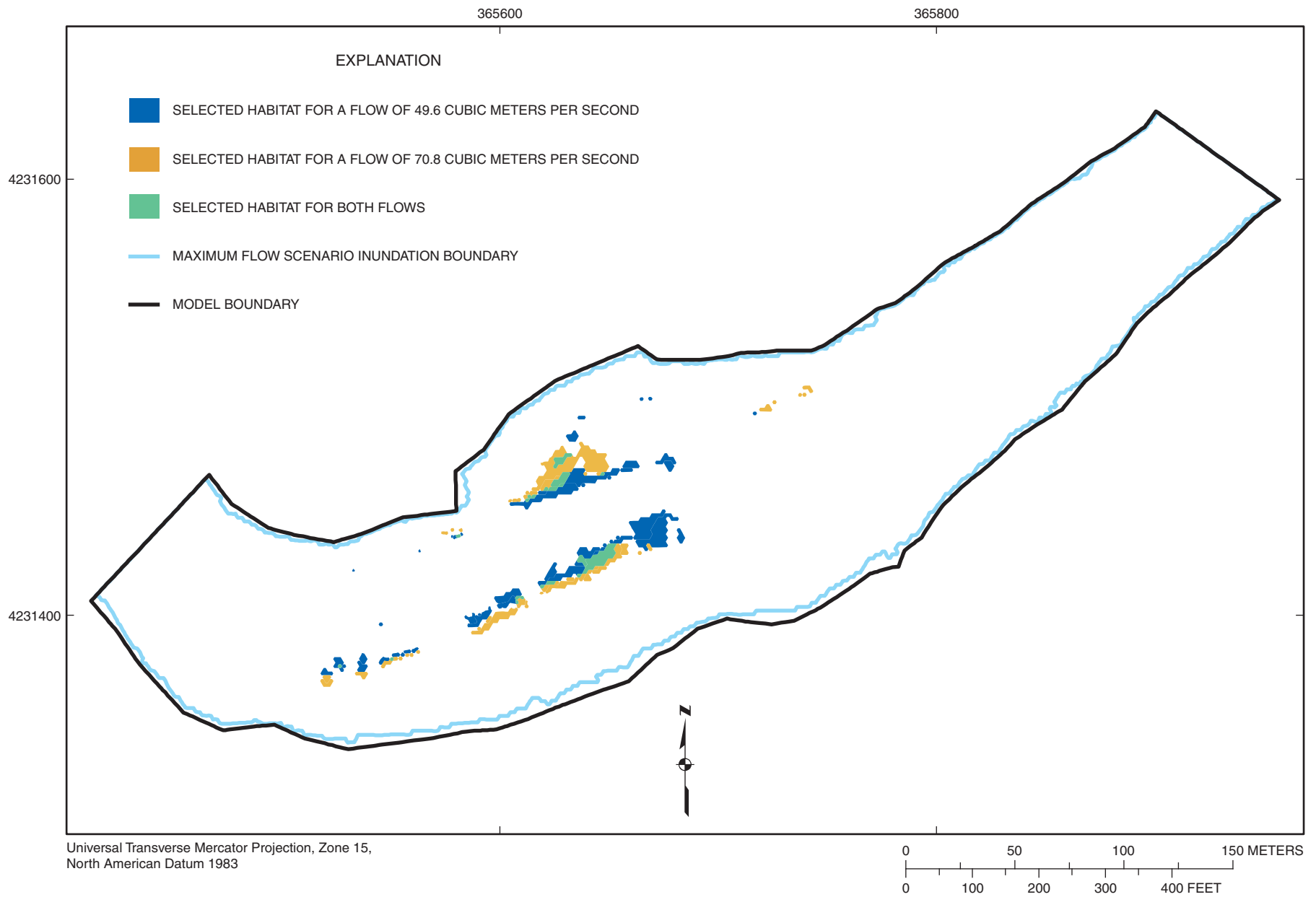
Figure 4-65. Selected habitat area distribution for habitat categories 16, 17 combined (channel catfish) at flows of 49.6 and 70.8 cubic meters per second at Marais des Cygnes River site MDC2.
